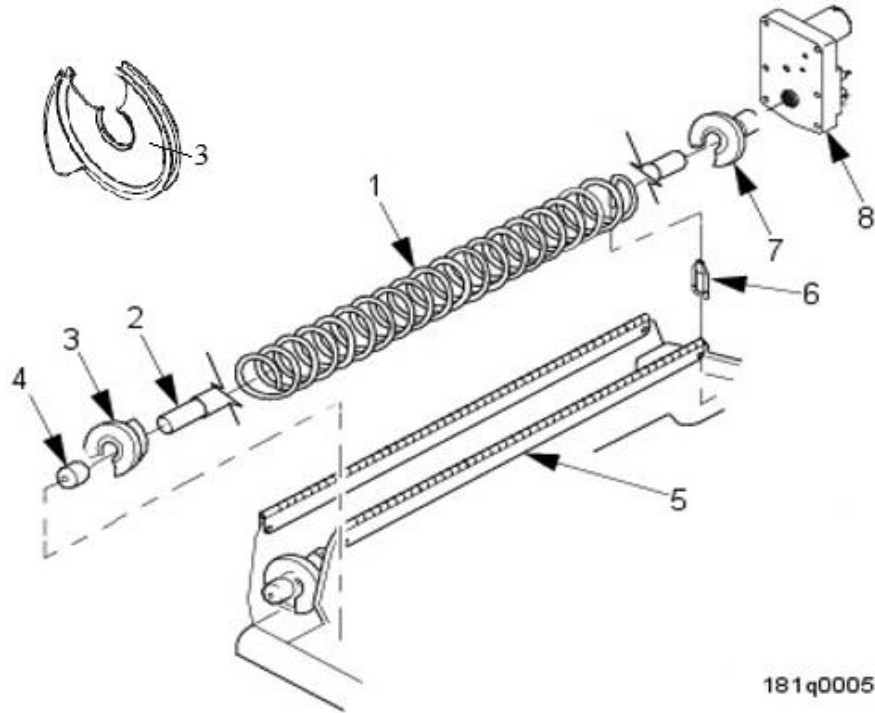
FIGURE 20: HALF CYCLE GUM & MINT SPIRAL ASSEMBLY
